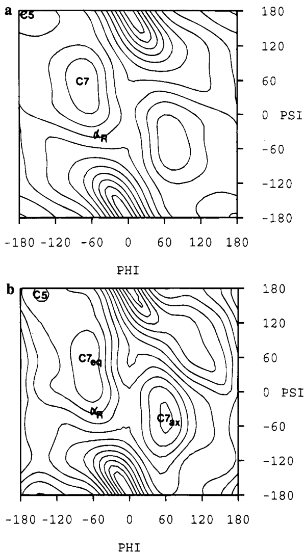
Figure 2. (a) The molecular mechanical ( \phi, \psi ) map for methyl-blocked glycylyl dipeptide generated using the force field presented here. Contours are drawn every 2 kcal/mol. (b) The molecular mechanical ( \phi, \psi ) map for methyl-blocked alanyl dipeptide generated using the force field presented here. Contours are drawn every 2 kcal/mol.
